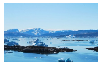
Arctic cycle
